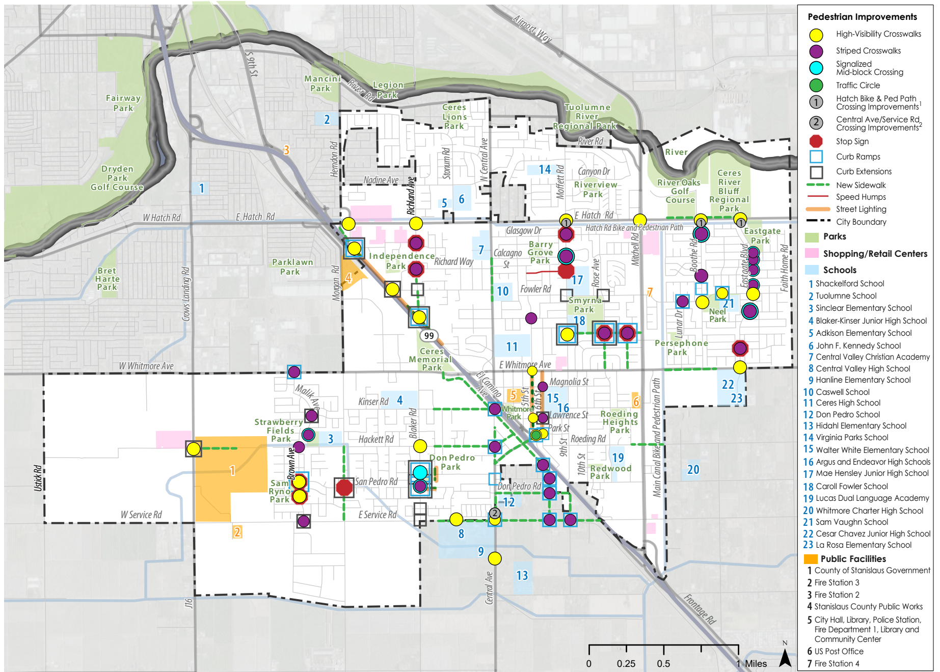
Figure X-X Planned Pedestrian Improvements
